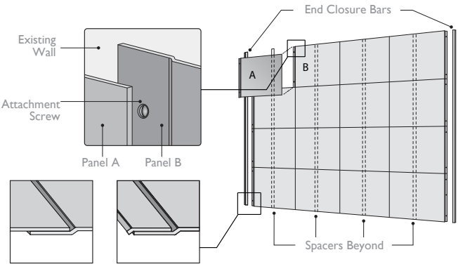
Terrace Wall Panels
