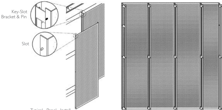
Key-Slot Wall Panels
