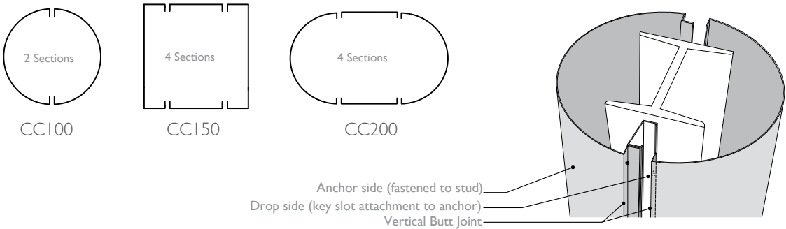
Column Sizes and System
