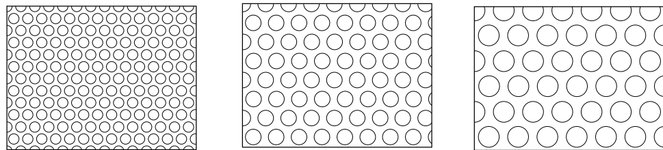
3/16" dia. 5/16" stg (33% open area) 1/4" dia. 3/8" stg (42% open area) 3/8" dia. 3/4" stg (17% open area)
