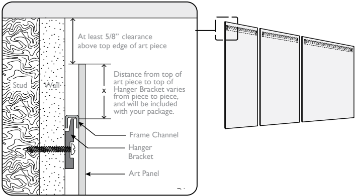
Blendz Installation Wall Hanging System
