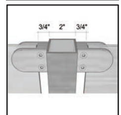
Panel Gripper
