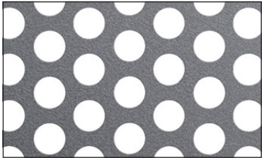
1/4" dia 3/8" stg | 40% open
