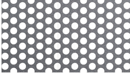
1/8" Diameter 3/16" Staggered Centers / 40% Open Area
