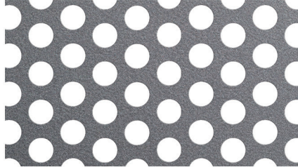
3/16" Diameter 5/16" Staggered Centers / 33% Open Area
