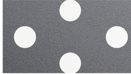
3/8" Diameter 3/4" Staggered Centers / 23% Open Area
