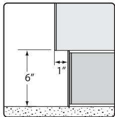
RC Recessed Capital/ RB Recessed Base 6" Standard height
