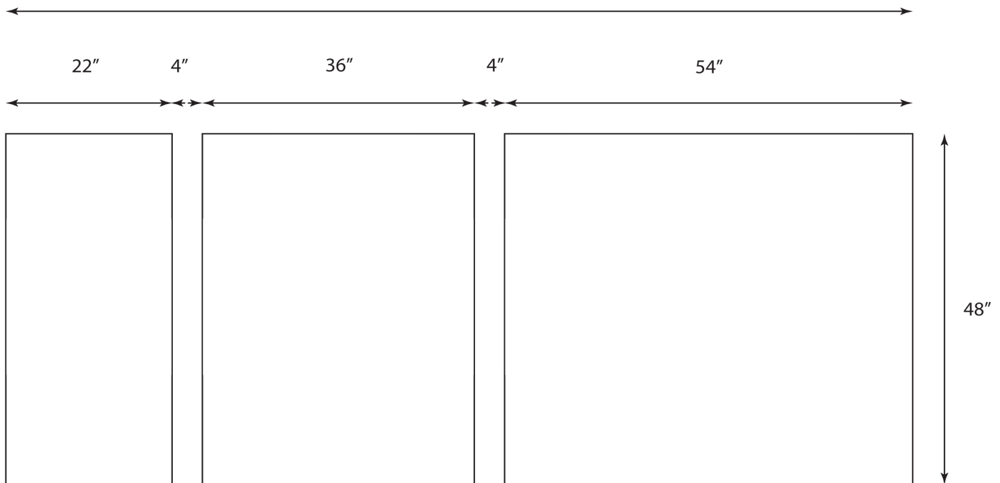
3 Piece Vertical Layout (4' x 10')
